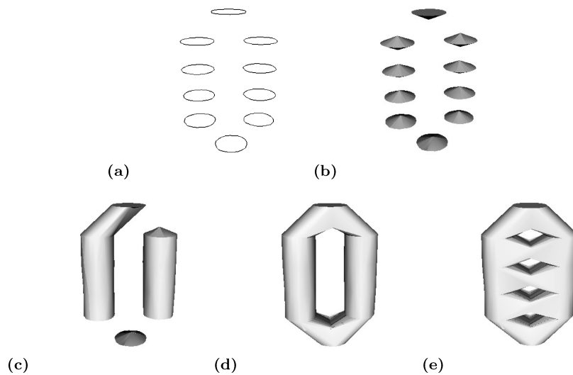
Fig. 11. Models generated from the contours in (a) for \beta equal to: (b) 0; (c) 1; (d) 3; (e) 5.
